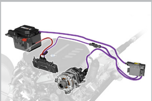
BMW 48V Mild Hybrid Technology
